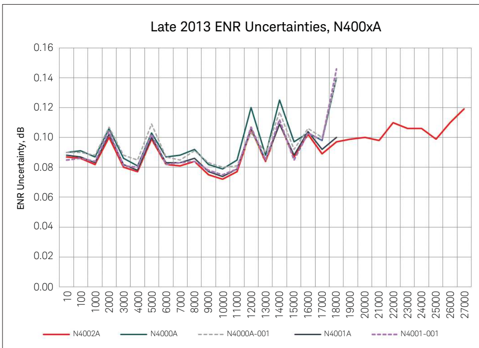
Figure 4. Characteristic ENR plot versus cardinal frequency points.
