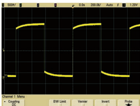
Under-compensated
