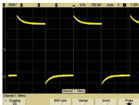
Over-compensated
