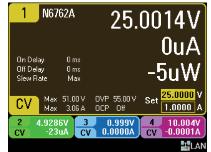
Figure 3. In Meter View, you can also view an enlarged view of one channel, displaying many settings and measured values, for that channel. A summary is shown for the other three channels.
